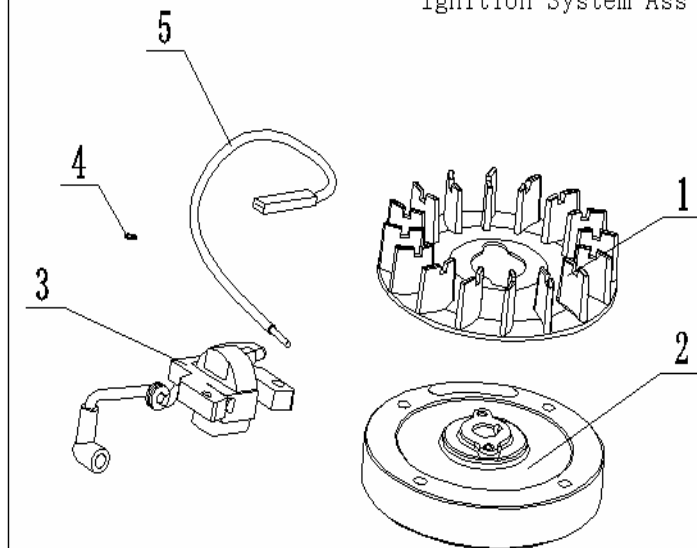
Ignition System Ass'y
