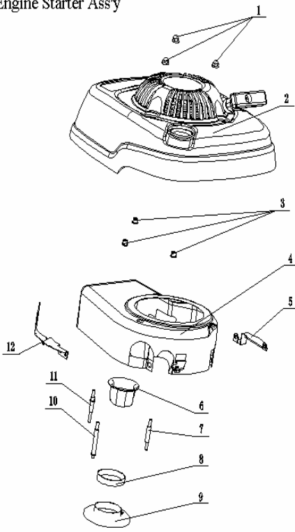
Engine Starter Ass'y
