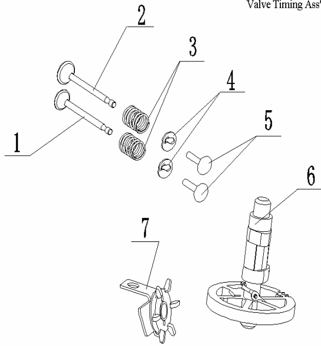
Valve Timing Ass'y
