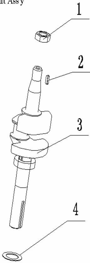
Crankshaft Ass'y
