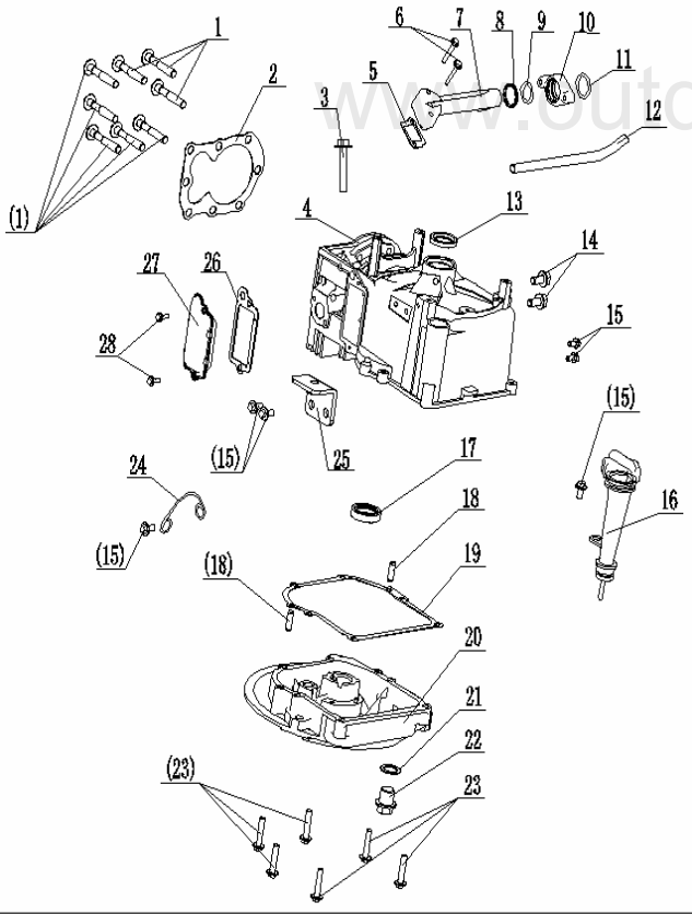
Crankcase Ass'y
